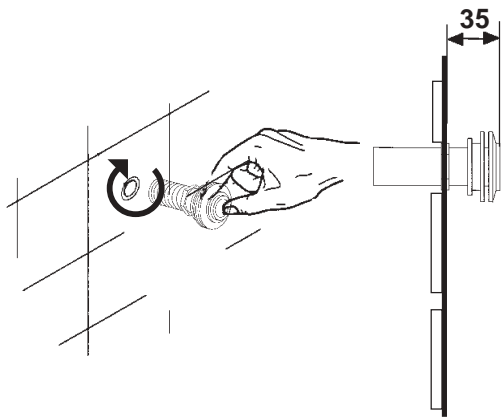
ALIMENTATION - WATER
