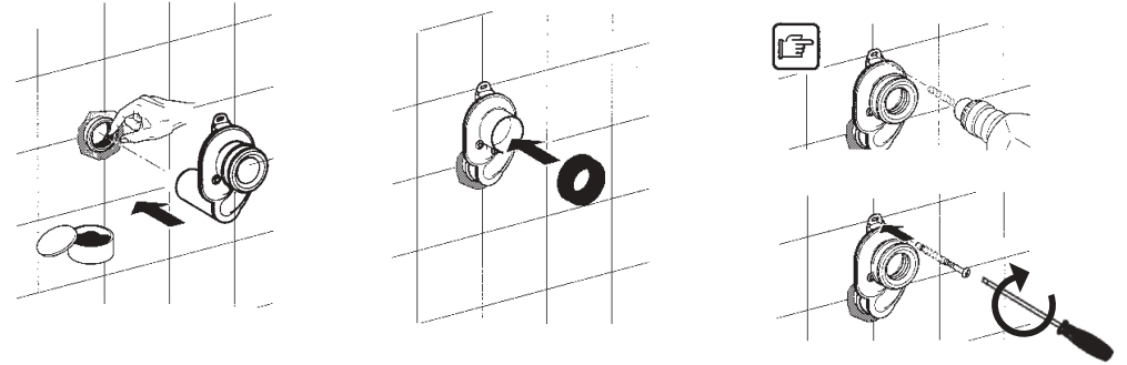
EVACUATION - OUTLET
